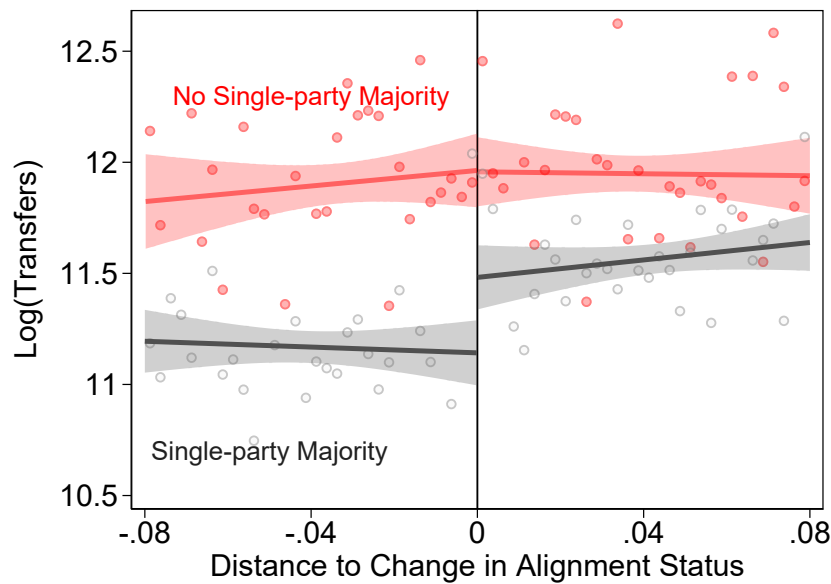
(B) LOG(TRANSFERS)
